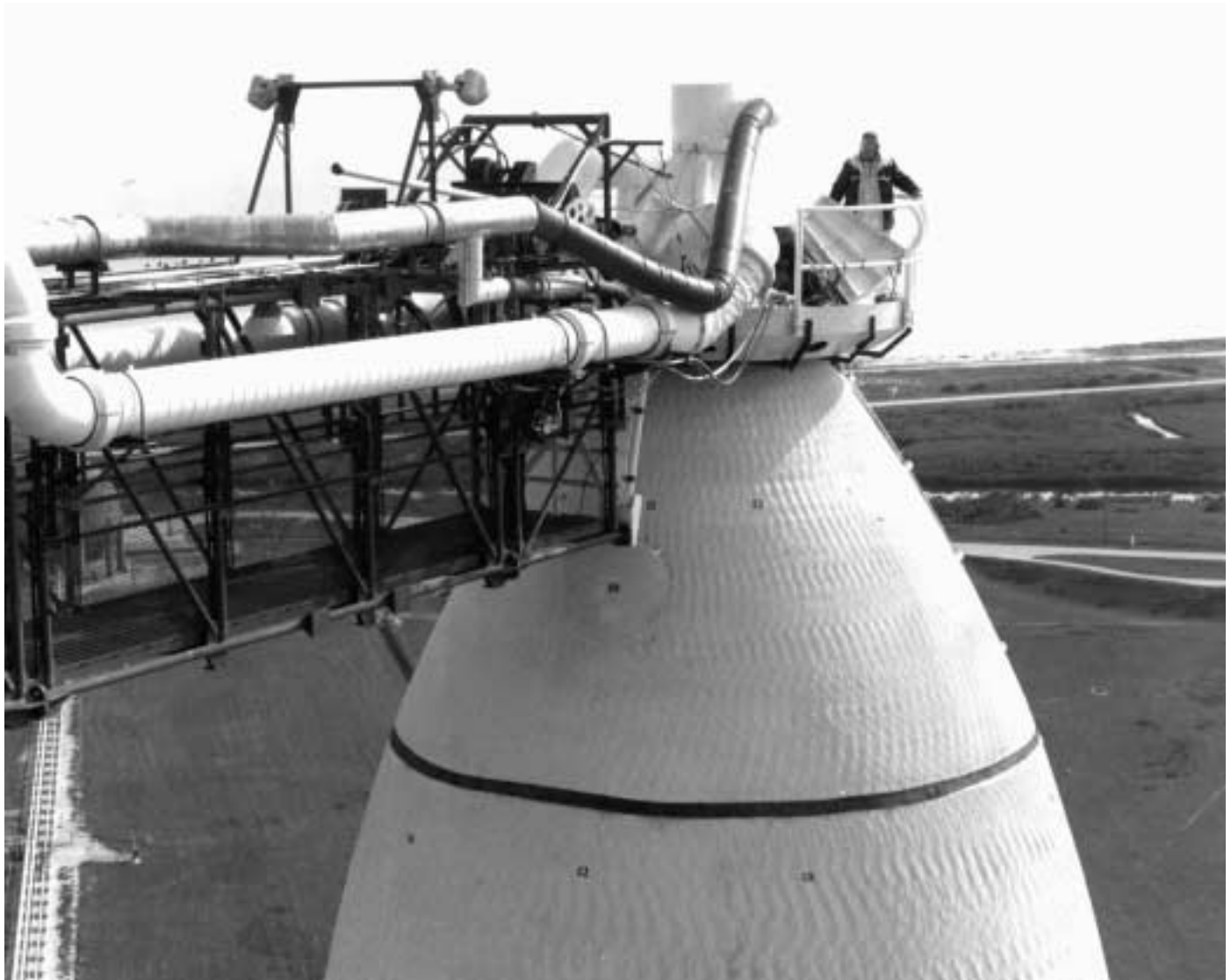
The gaseous oxygen vent hood, known as the "beanie cap," is located on the end of the highest swingarm attached to the Fixed Service Structure.
