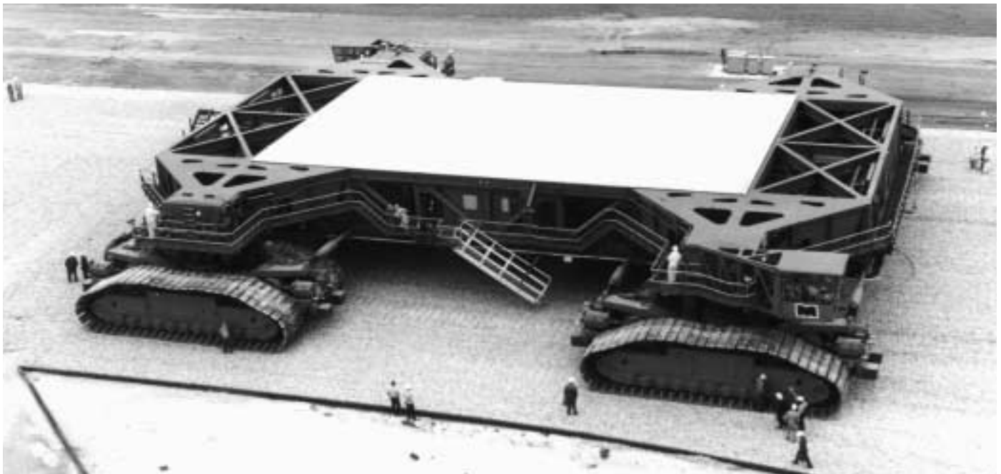
The Crawler-Transporter can lift the Space Shuttle on its Mobile Launcher Platform and move it to and from the launch pads.
